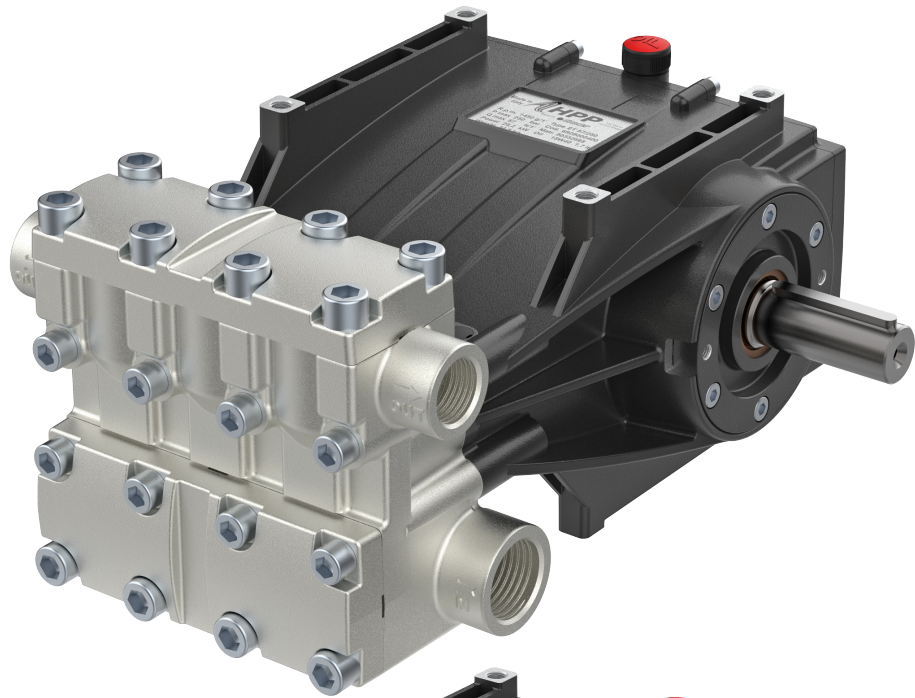
LQ HEAD
