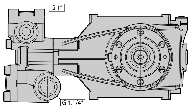
LQ HEAD
