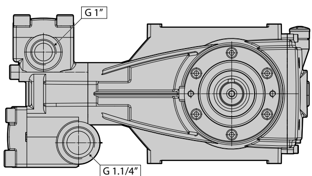
MQ HEAD
