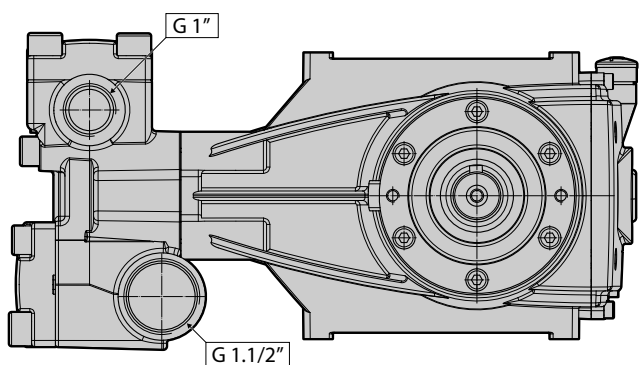
HQ HEAD
